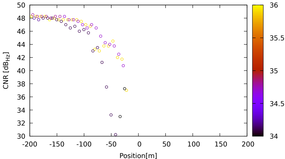
CNR vs position for G22 (L1) on LeicaGS18 - DOY 263 jam. 2
