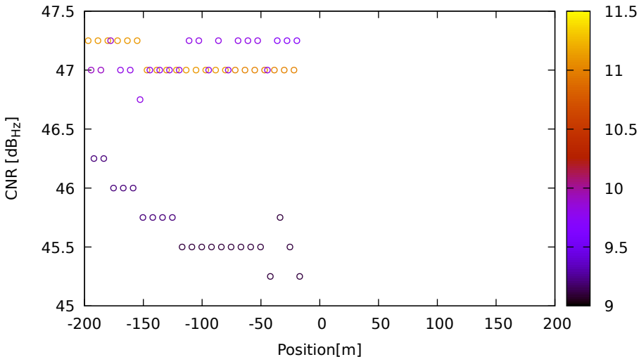
CNR vs position for G32 (L5) on LeicaGS18 - DOY 263 jam. 2
