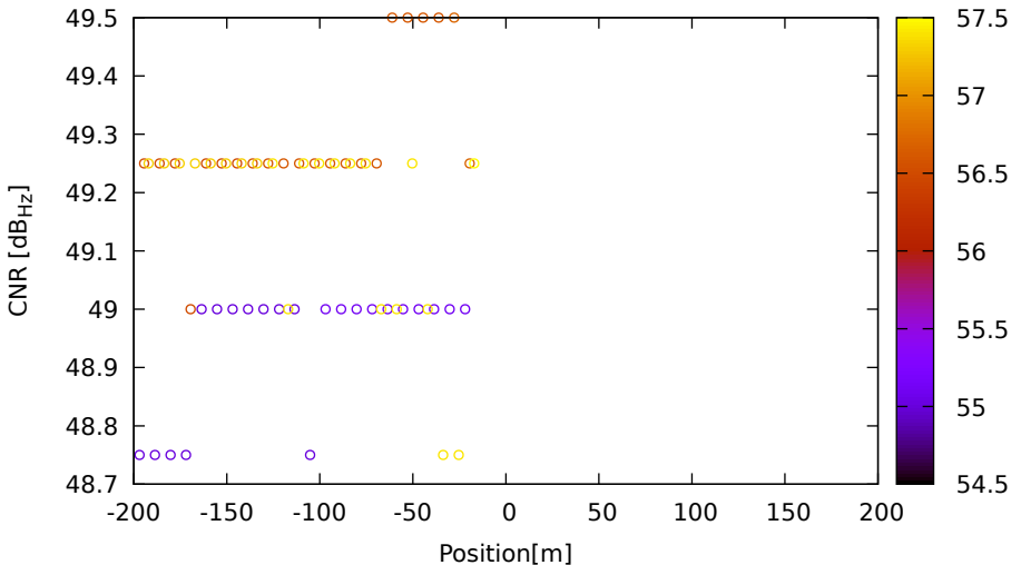
CNR vs position for R02 (G2) on LeicaGS18 - DOY 263 jam. 2
