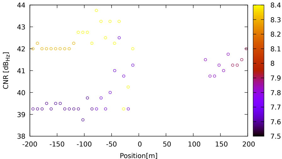
CNR vs position for R03 (G1) on LeicaGS18 - DOY 263 jam. 3
