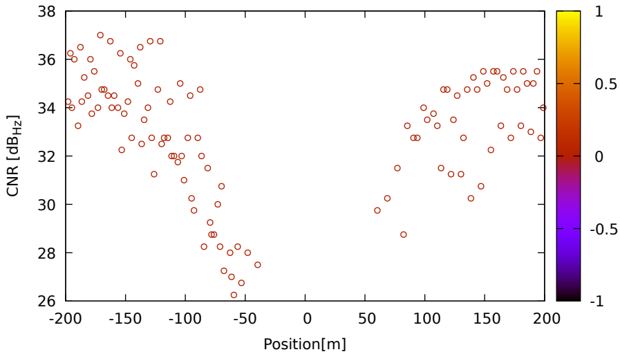
CNR vs position for R09 (G1) on LeicaGS18 - DOY 263 jam. 1
