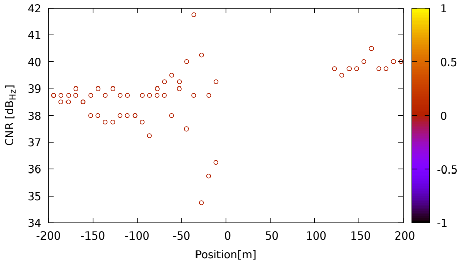
CNR vs position for R09 (G1) on LeicaGS18 - DOY 263 jam. 3
