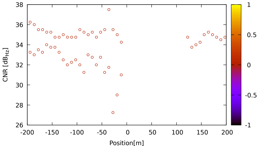
CNR vs position for R10 (G1) on LeicaGS18 - DOY 263 jam. 3
