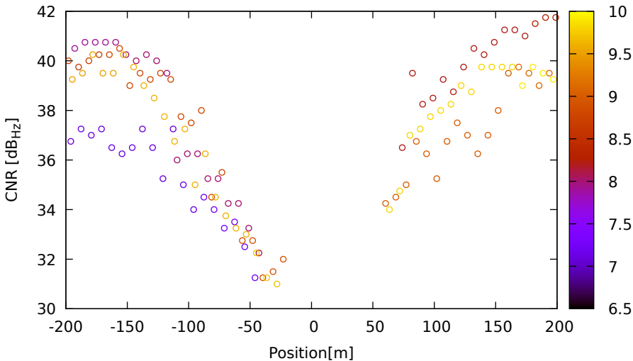
CNR vs position for R18 (G2) on LeicaGS18 - DOY 263 jam. 1
