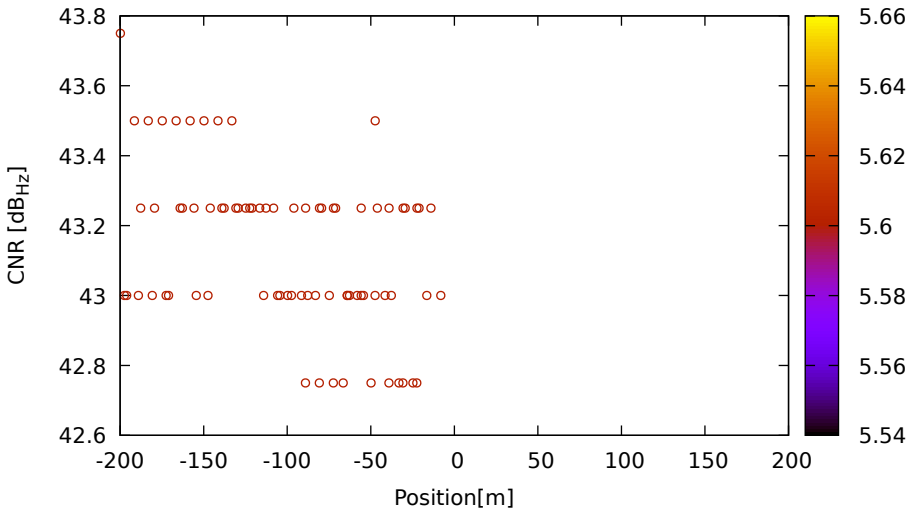
CNR vs position for C02 (B2) on LeicaGS18 - DOY 263 jam. 2
