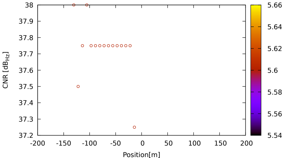
CNR vs position for C02 (B3) on LeicaGS18 - DOY 263 jam. 3
