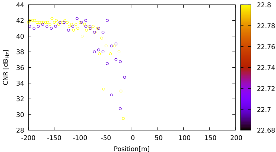
CNR vs position for C05 (B1) on LeicaGS18 - DOY 263 jam. 2
