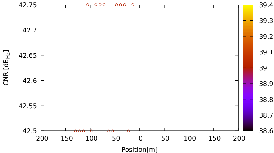
CNR vs position for C09 (B3) on LeicaGS18 - DOY 263 jam. 3
