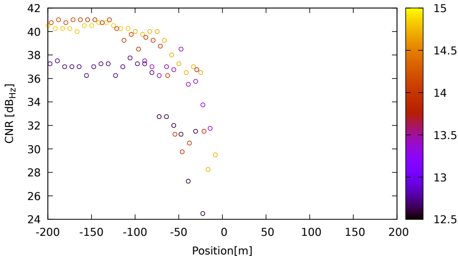
CNR vs position for C12 (B1) on LeicaGS18 - DOY 263 jam. 2
