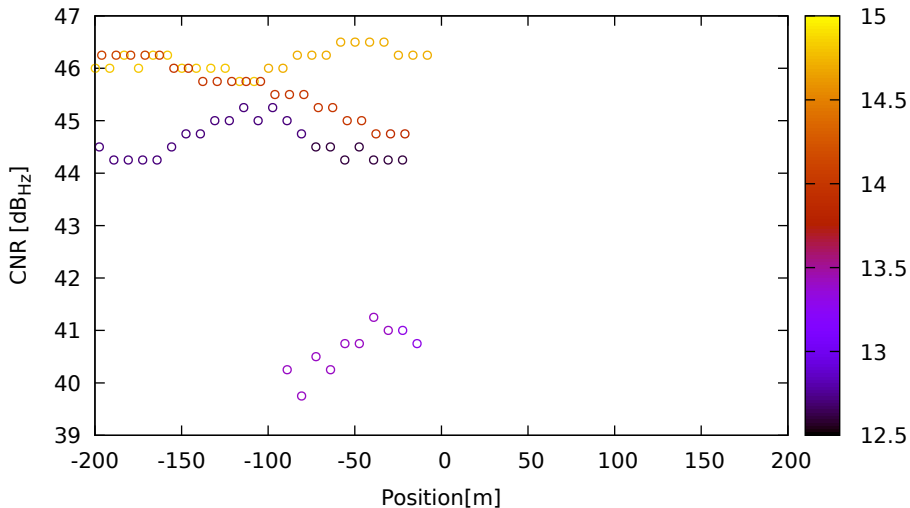
CNR vs position for C12 (B2) on LeicaGS18 - DOY 263 jam. 2
