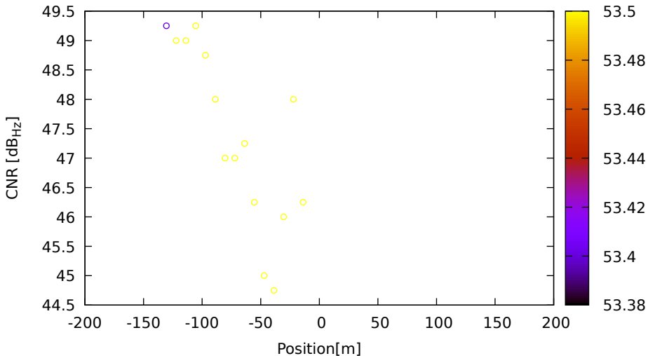
CNR vs position for C14 (B1) on LeicaGS18 - DOY 263 jam. 3
