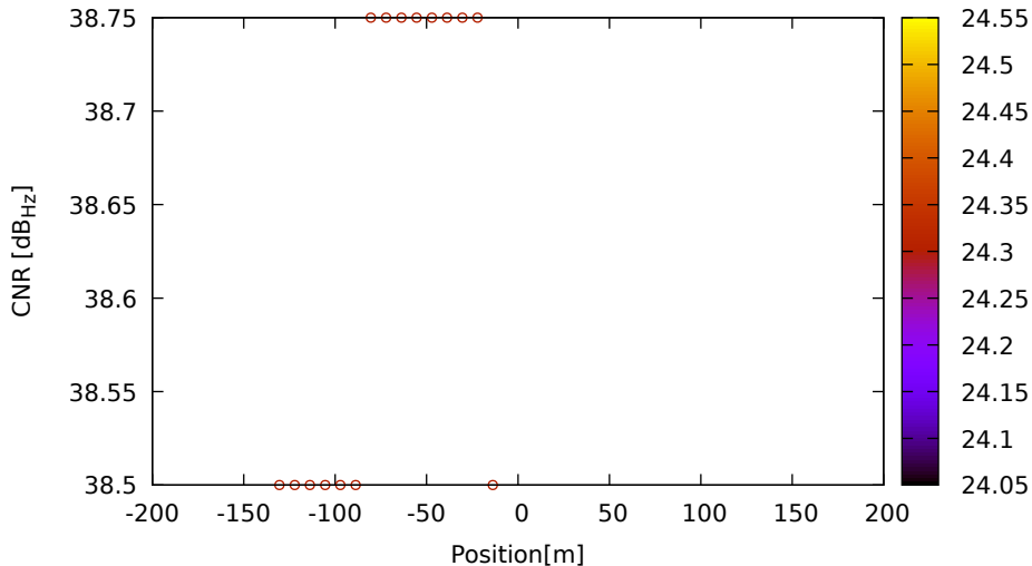
CNR vs position for C16 (B3) on LeicaGS18 - DOY 263 jam. 3
