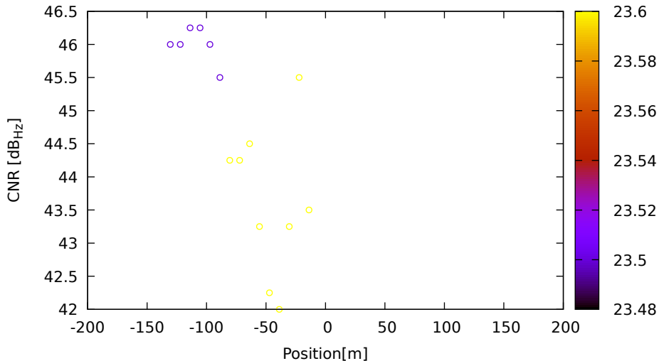
CNR vs position for C28 (B1) on LeicaGS18 - DOY 263 jam. 3
