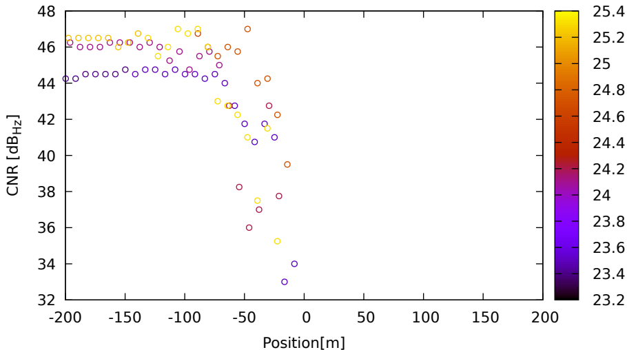
CNR vs position for C33 (B1) on LeicaGS18 - DOY 263 jam. 2
