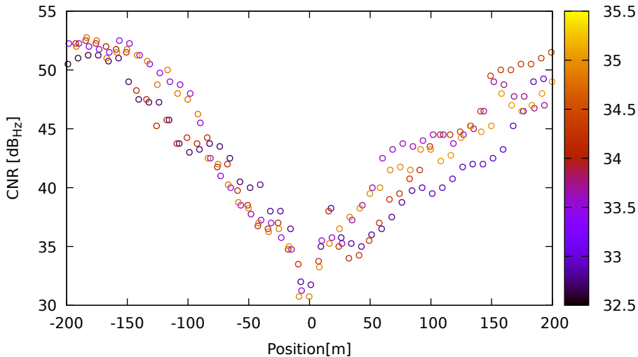
CNR vs position for E04 (E5) on LeicaGS18 - DOY 263 jam. 1
