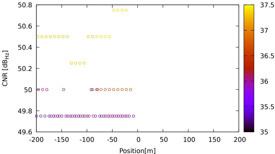
CNR vs position for E04 (E5a) on LeicaGS18 - DOY 263 jam. 2
