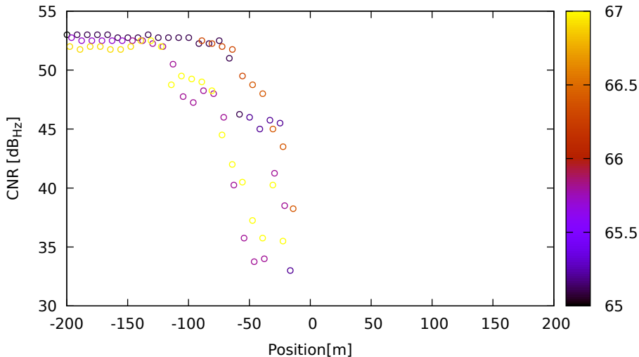
CNR vs position for E10 (E1) on LeicaGS18 - DOY 263 jam. 2
