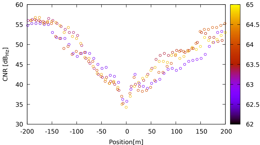
CNR vs position for E10 (E5) on LeicaGS18 - DOY 263 jam. 1
