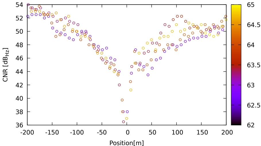
CNR vs position for E10 (E5b) on LeicaGS18 - DOY 263 jam. 1
