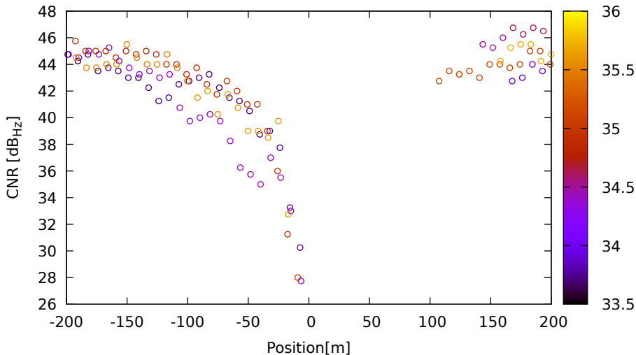
CNR vs position for E11 (E1) on LeicaGS18 - DOY 263 jam. 1
