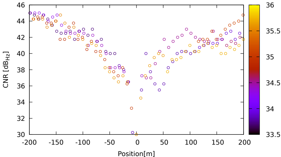
CNR vs position for E11 (E5a) on LeicaGS18 - DOY 263 jam. 1
