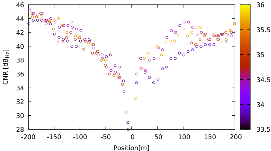
CNR vs position for E11 (E5b) on LeicaGS18 - DOY 263 jam. 1
