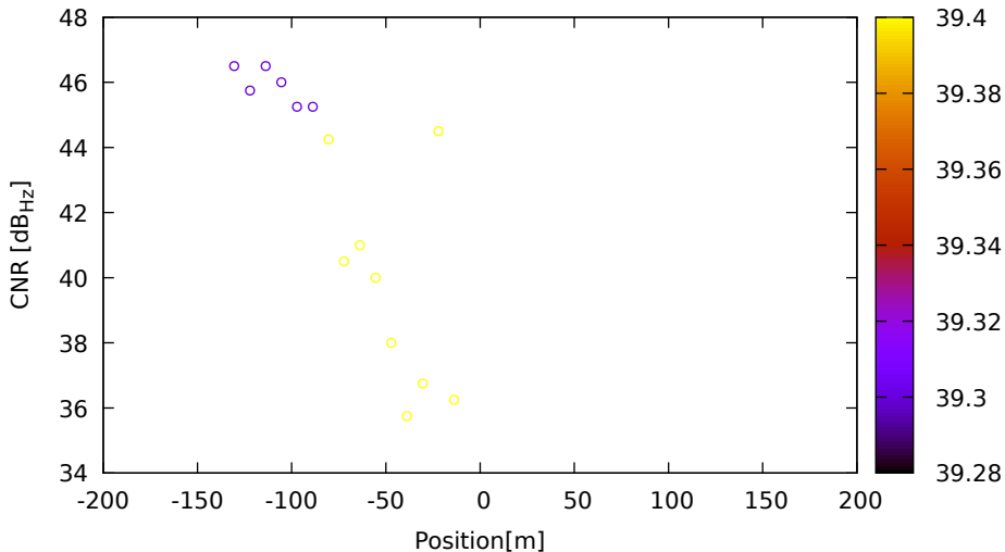
CNR vs position for G04 (L2) on LeicaGS18 - DOY 263 jam. 3
