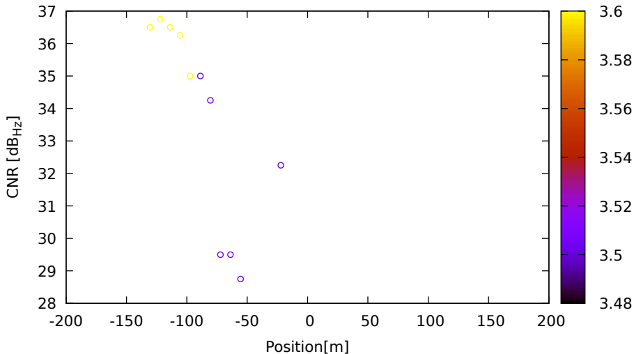
CNR vs position for G08 (L1) on LeicaGS18 - DOY 263 jam. 3
