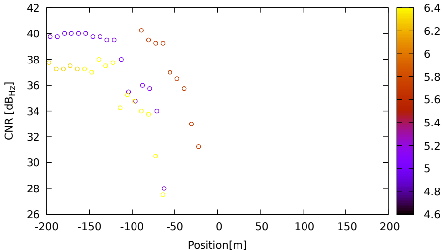
CNR vs position for G09 (L1) on LeicaGS18 - DOY 263 jam. 2
