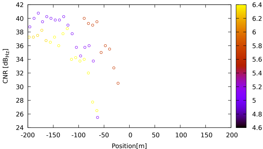
CNR vs position for G09 (L2) on LeicaGS18 - DOY 263 jam. 2
