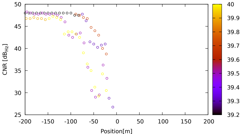
CNR vs position for G17 (L1) on LeicaGS18 - DOY 263 jam. 2
