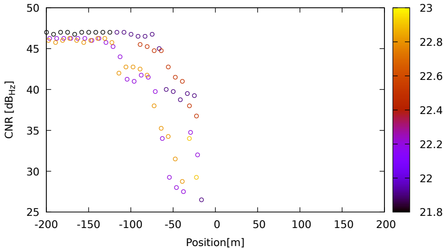
CNR vs position for G31 (L1) on LeicaGS18 - DOY 263 jam. 2
