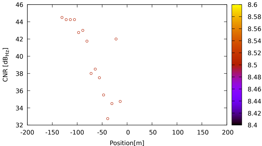
CNR vs position for G32 (L1) on LeicaGS18 - DOY 263 jam. 3
