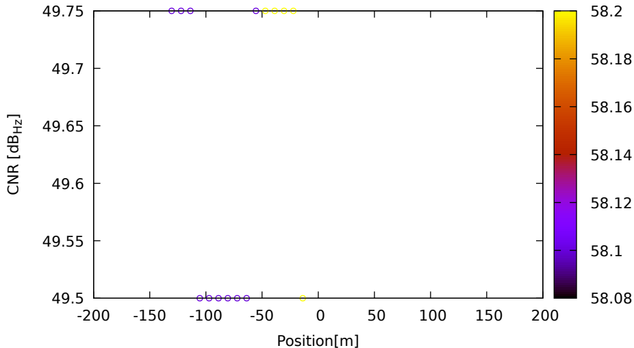
CNR vs position for R02 (G2) on LeicaGS18 - DOY 263 jam. 3
