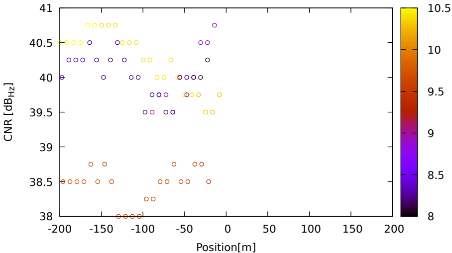
CNR vs position for R08 (G2) on LeicaGS18 - DOY 263 jam. 2
