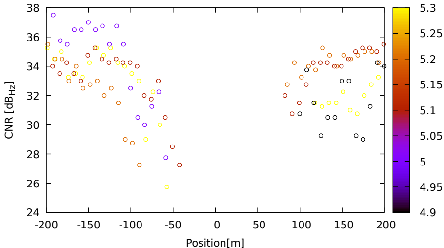
CNR vs position for R09 (G1) on LeicaGS18 - DOY 263 jam. 1
