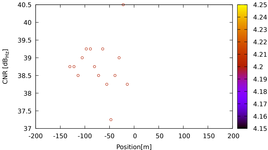
CNR vs position for R09 (G1) on LeicaGS18 - DOY 263 jam. 3
