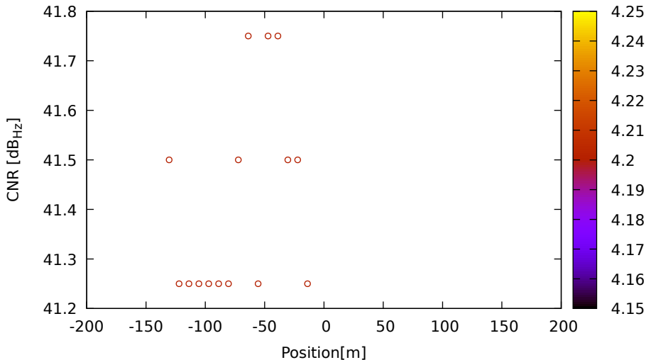
CNR vs position for R09 (G2) on LeicaGS18 - DOY 263 jam. 3
