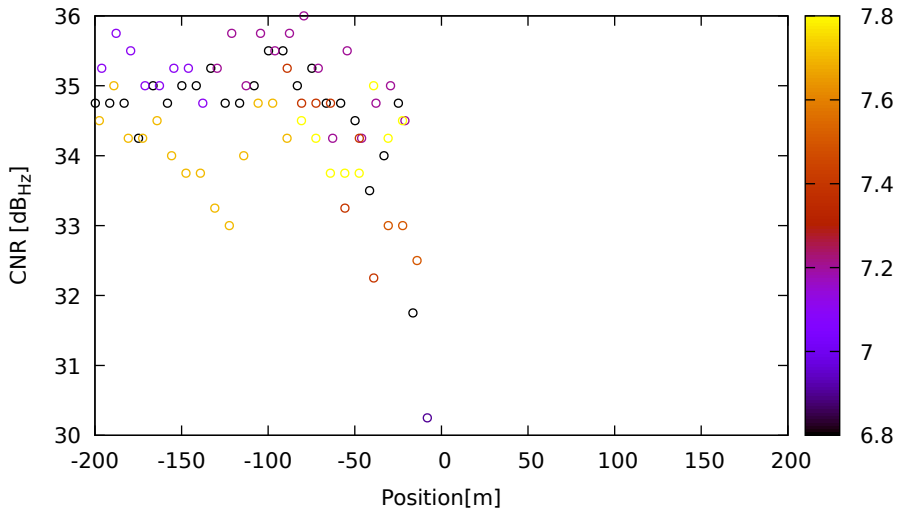
CNR vs position for R10 (G1) on LeicaGS18 - DOY 263 jam. 2
