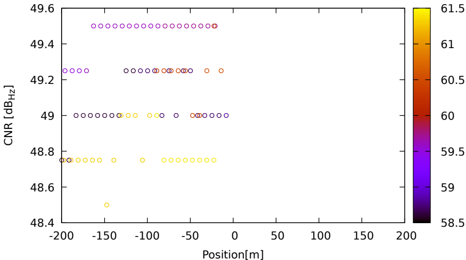
CNR vs position for R17 (G2) on LeicaGS18 - DOY 263 jam. 2
