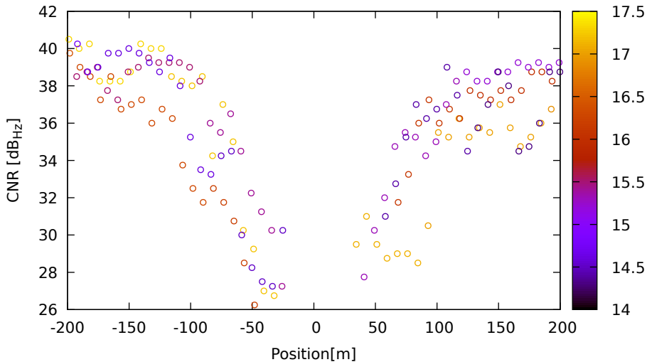
CNR vs position for R23 (G1) on LeicaGS18 - DOY 263 jam. 1
