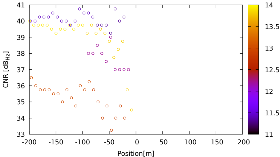
CNR vs position for R23 (G1) on LeicaGS18 - DOY 263 jam. 2
