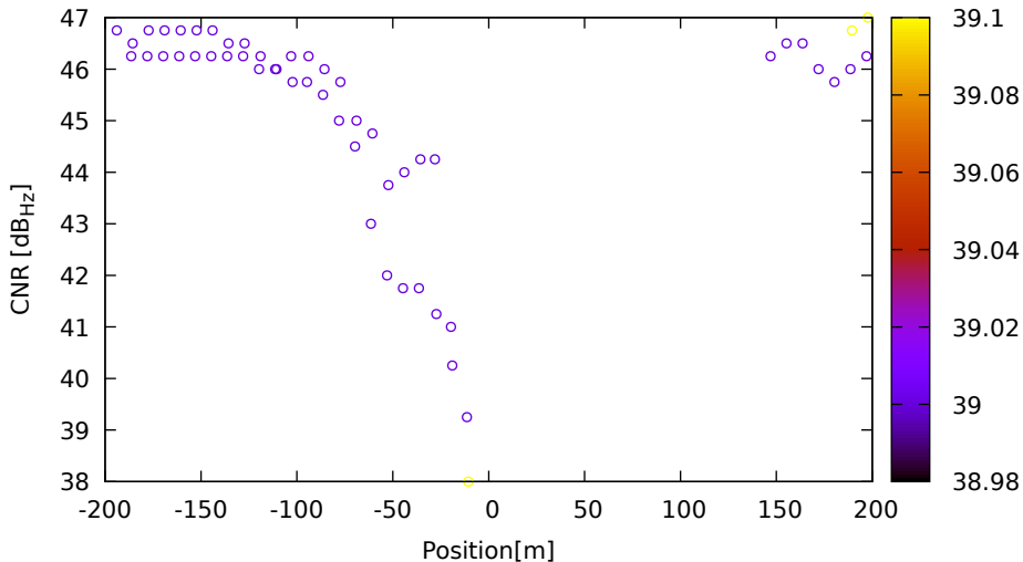
CNR vs position for C09 (B1) on LeicaGS18 - DOY 263 jam. 3
