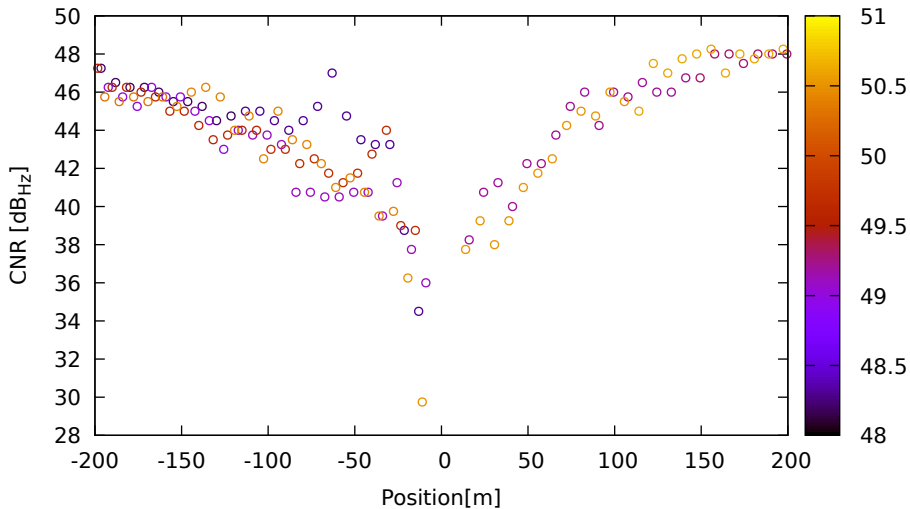
CNR vs position for C14 (B1) on LeicaGS18 - DOY 263 jam. 1
