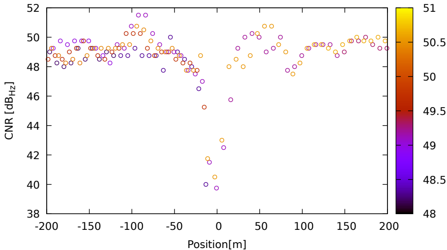
CNR vs position for C14 (B3) on LeicaGS18 - DOY 263 jam. 1
