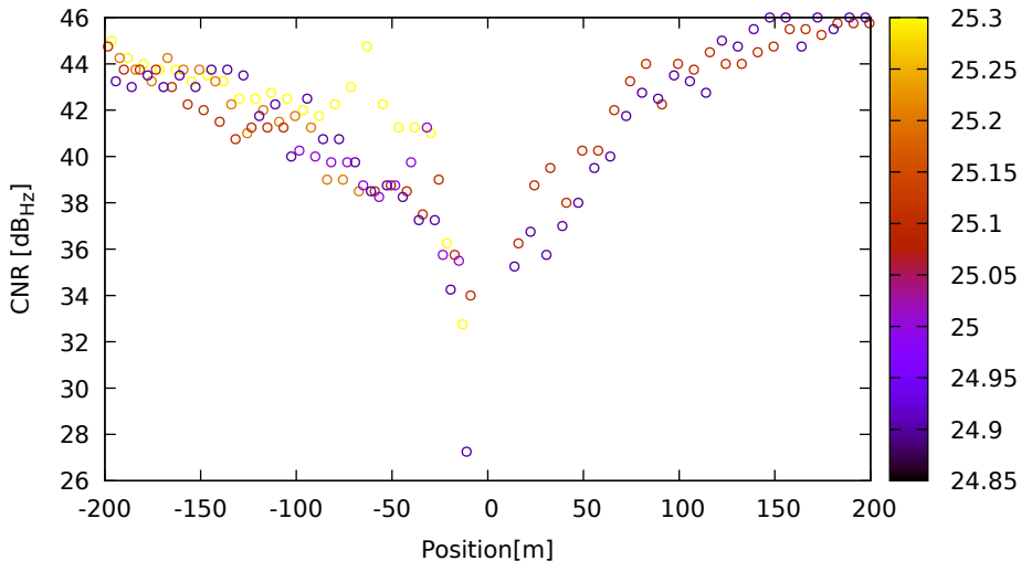
CNR vs position for C16 (B1) on LeicaGS18 - DOY 263 jam. 1
