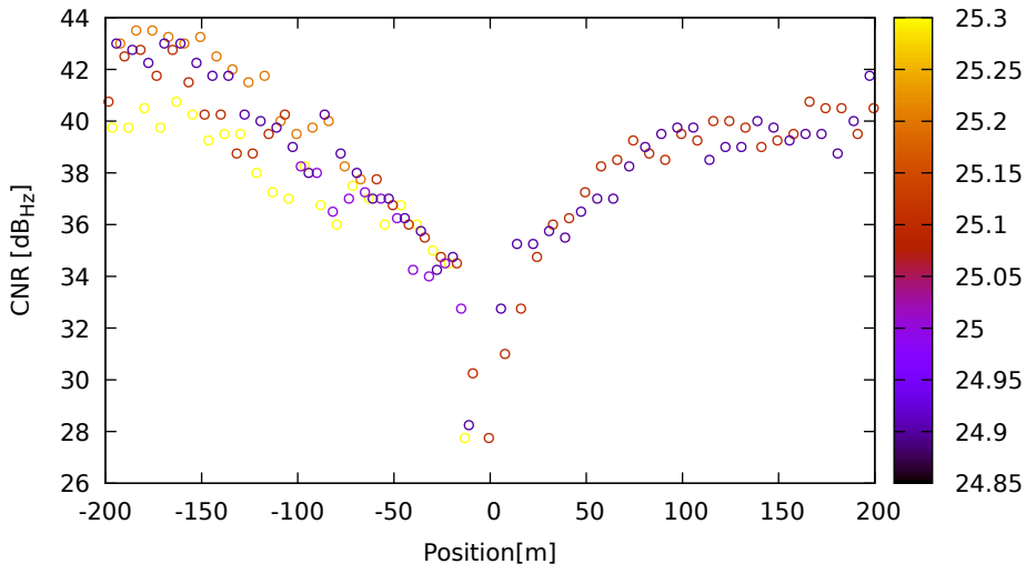
CNR vs position for C16 (B2) on LeicaGS18 - DOY 263 jam. 1
