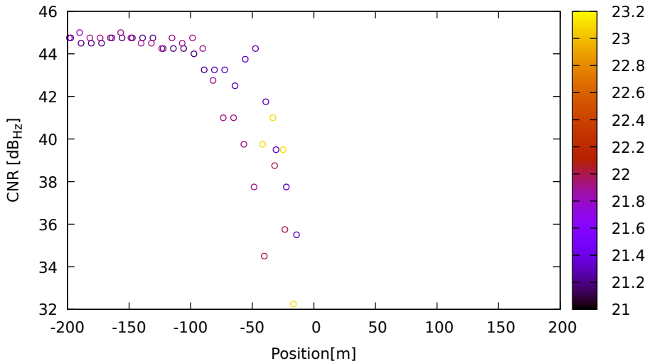
CNR vs position for C28 (B1) on LeicaGS18 - DOY 263 jam. 2
