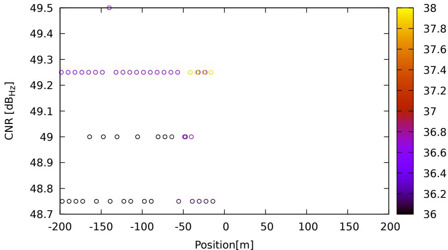
CNR vs position for E11 (E5) on LeicaGS18 - DOY 263 jam. 2
