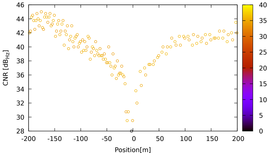
CNR vs position for E11 (E5b) on LeicaGS18 - DOY 263 jam. 1
